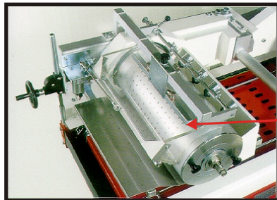
Aluminium Sowing roller & stainless steel nozzels.
